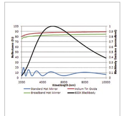
NIR/FIR Reflectance of Standard Hot Mirror, ITO, and Broadband Hot Mirror (normal incidence)
