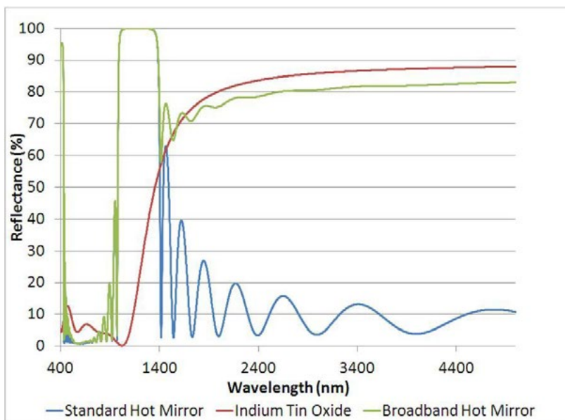
Figure 4. Top- the Broadband Hot Mirror (green) is composed of a Standard Hot mirror (blue) with an infrared reflector (red) on the back side
