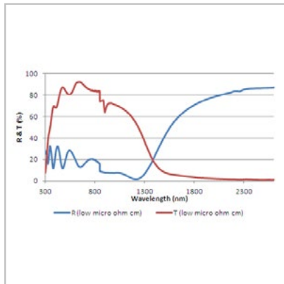
VIS/NIR R&T of Metallic Beamsplitter (AOI = 45 deg)
