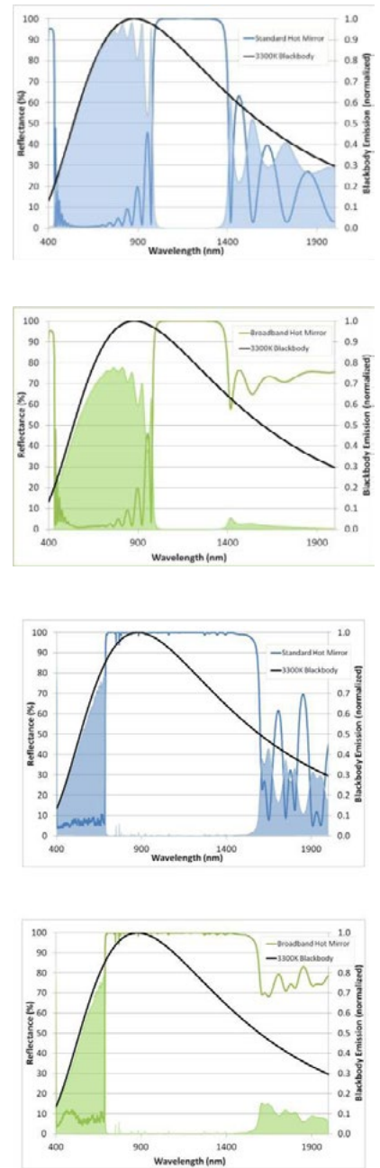
Figure 2. Blue curves- 3300 K blackbody curve (black) with two different hot mirrors (dark blue). Green curves- 3300 K blackbody curve (black) with two different Omega Broadband Hot Mirrors (dark green). Shaded areas indicate light that passes through the filter. Note that very little light is transmitted through Omega's filter at higher IR wavelengths.
