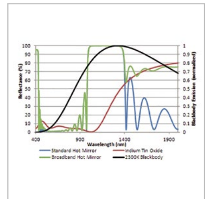
VIS/NIR Reflectance of Standard Hot Mirror, ITO and Broadband Hot Mirror (normal incidence)
