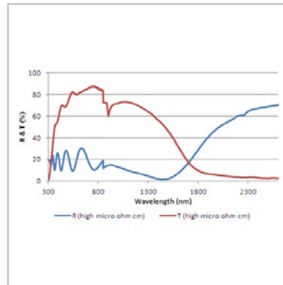
NIR/IR R&T of Metallic Beamsplitter (AOI = 45 deg)
