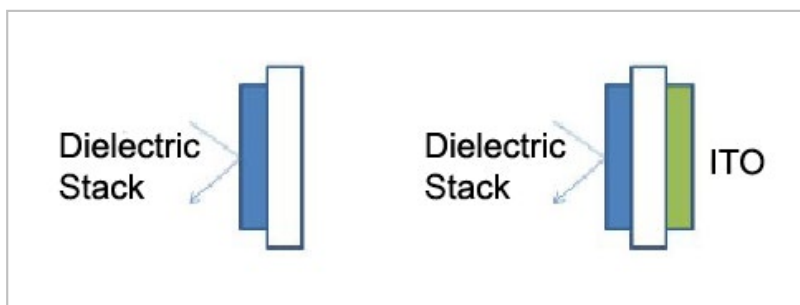
Schematic of Standard Hot Mirror (left) and Broadband Hot Mirror (right)
