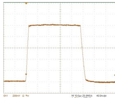
Current monitor output, scale: 20A/Div
