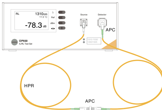
Figure 7: After the IL reference has been completed, the DUT can be connected as normal.
