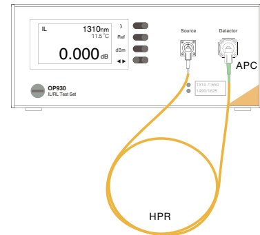
Figure 6: Once the reflector stub is removed, the HPR can be connected to the detector for an IL reference.
