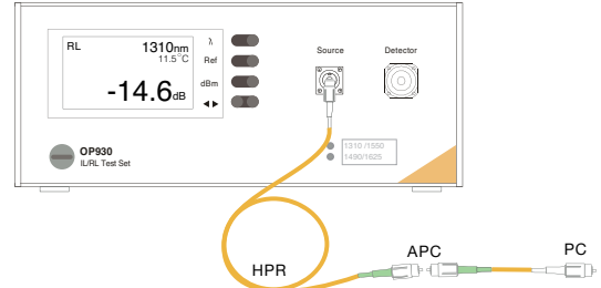
Figure 4: Instead of using a substitute cable, this method utilizes a short reflector stub to create a large reflection near the end of the HPR.
