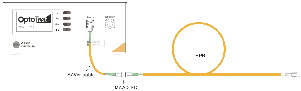
Figure 3: SAVer cable connected to High Performance Cable
