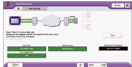
J-QuickCheck configuration page and results
