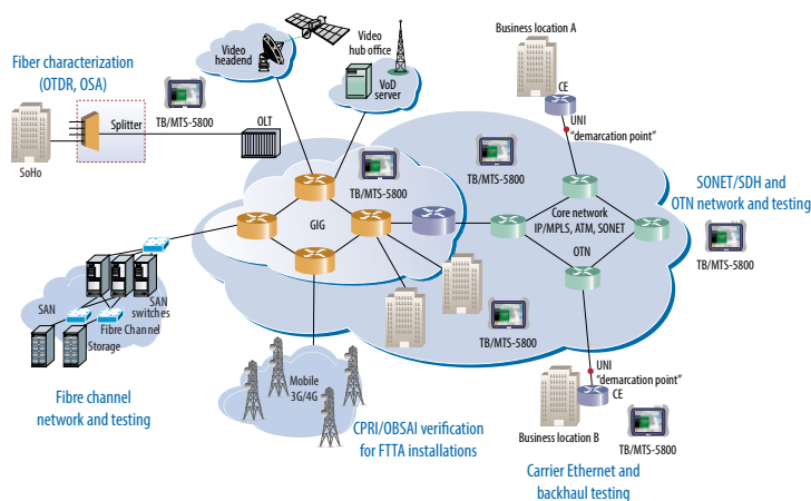
Figure 1. T-BERD/MTS-5800 in the carrier Ethernet network
