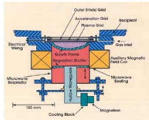
Figure 2. With ion-assisted deposition and electron cyclotron resonance, particles move at a much higher average speed on their way to the substrate.
