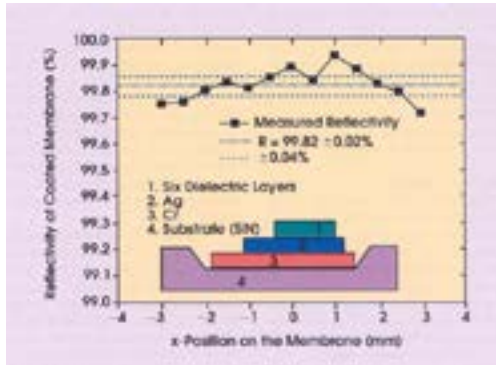
Figure 3. A piezoelectrically deformable foil with a coating of silver and six layers of dielectric coating is optimized for 1064 nm.
