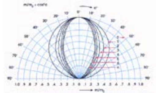
Figure 4. This illustrates the radial symmetric thickness distribution of a coating at rotation of the substrate during the coating process. The characteristics of an area evaporation source: a is the angle between the viewing direction and the symmetry axis of the evaporation source; m/m_0 is the under angle a emitted mass, normalized to the under a = 0^\circ emitted mass. The exponent n determines the shape of the vapor clouds: The bigger the n , the more directed is the cloud and the less material is emitted at greater angles.
