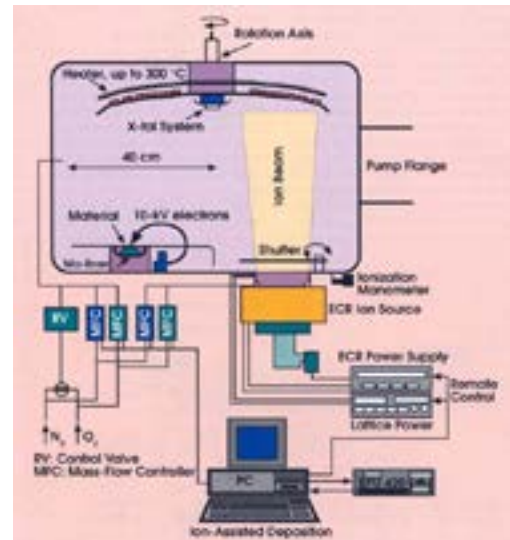
Figure 1. In the typical ion-beam-supported vapor deposition equipment setup, the relatively low thermal particle energy of about 0.1 eV dissipates quickly.
