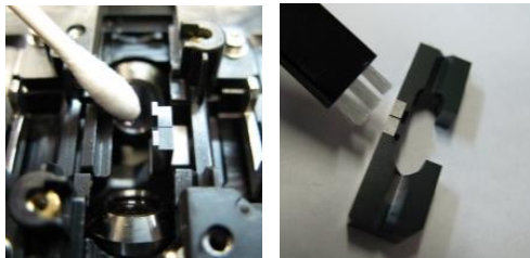
Detachable V-groove and Easy Cleaning
