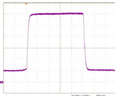
Figure: Current monitor output, scale: 40A/Div
