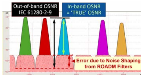
Out-of-band versus 'True' in-band OSNR in ROADM networks
