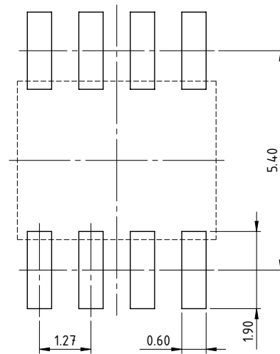
RECOMMENDED PCB-FOOTPRINT
