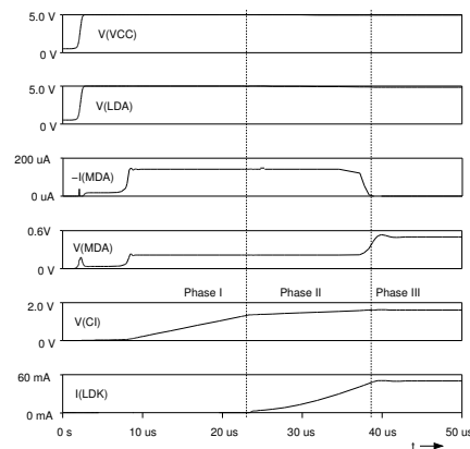
Figure 1: Turn-on behaviour
