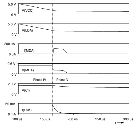
Figure 2: Turn-off behaviour
