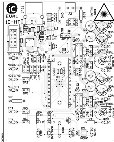
Figure 1: Component side (size 100 mm x 80 mm)
