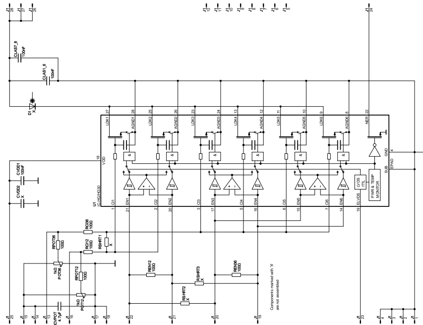
Figure 5: Circuit diagram
