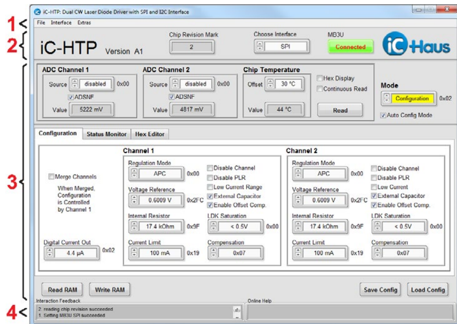
Figure 3: iC-HTP evaluation software
