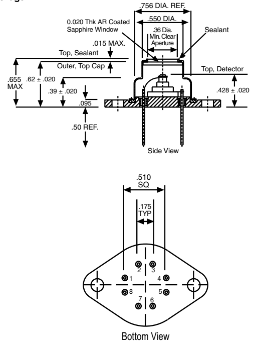
3CN Package
