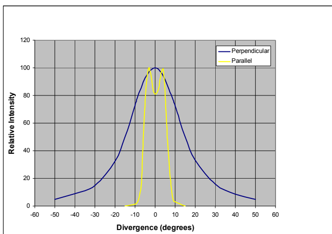
Figure 5: Beam divergence parallel and perpendicular to the junction plane
