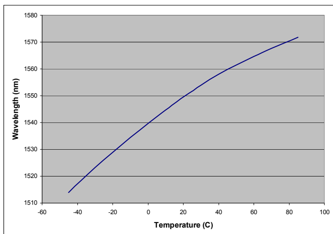
Figure 1: Wavelength vs. Temperature
