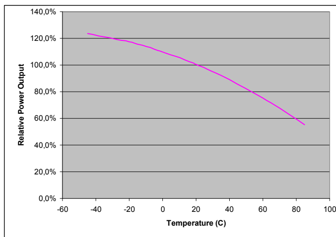
Figure 4: Peak Optical Output Power vs. Temperature
