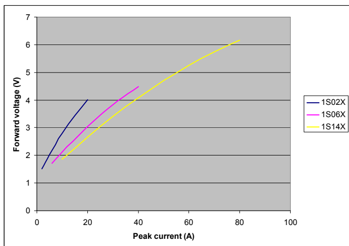
Figure 3: Static Forward Voltage vs. Peak Current
