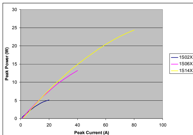
Figure 2: Optical Output Power vs. Forward Current
