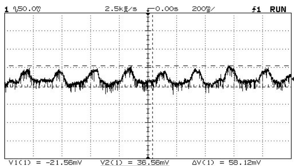
Measured ripple for dBC-380-5x at V_{out} = 370\text{ Vdc} Ripple: ca. 1.6 \cdot 10^{-4}
