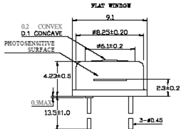
Pinout & Mechanical Dimensions (mm)
