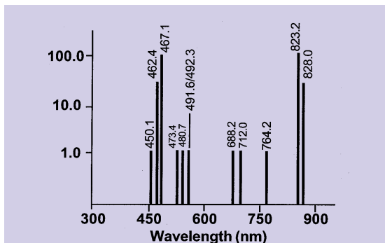
XENON SPECTRUM
