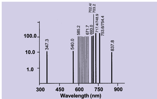
NEON SPECTRUM
