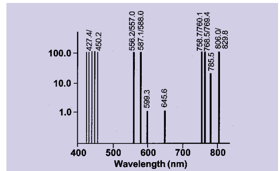
KRYPTON SPECTRUM
