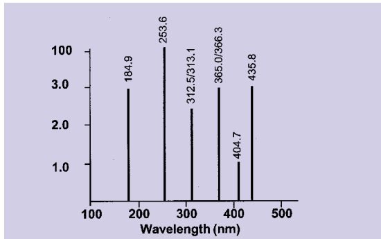
MERCURY SPECTRUM
