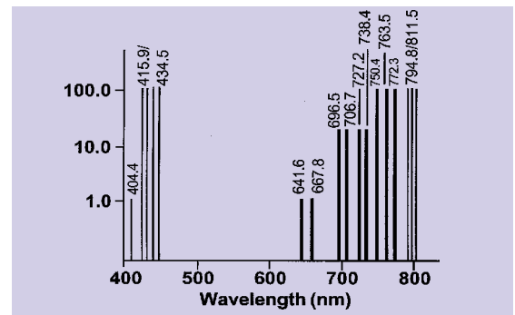
ARGON SPECTRUM
