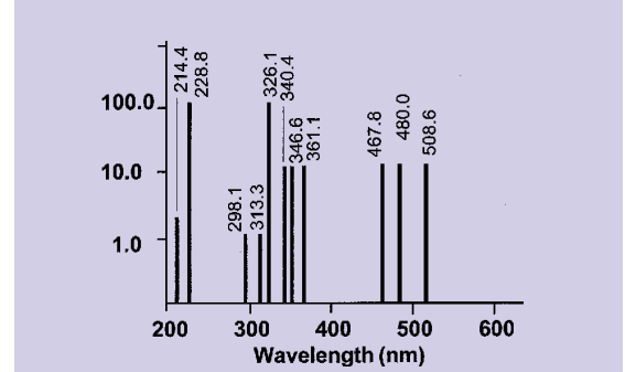
CADMIUM SPECTRUM
