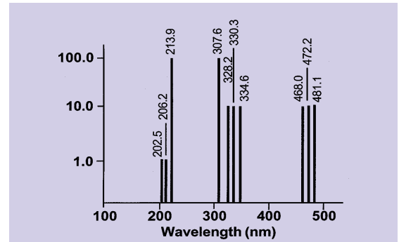
ZINC SPECTRUM
