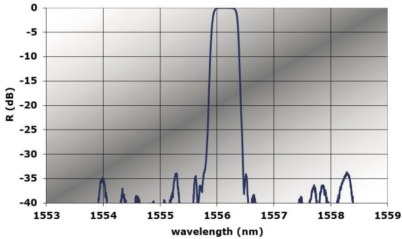
Reflection Spectrum
