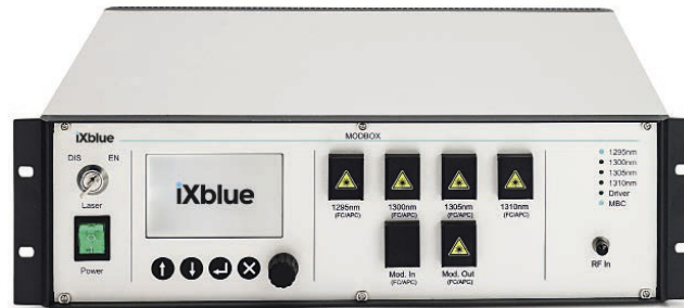
4 lanes Laser ModBox - NRZ example - Front panel
