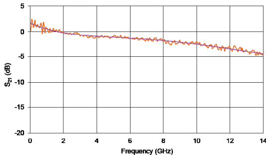
NIR-MX800-LN-10 Typical S_{21} Curve
