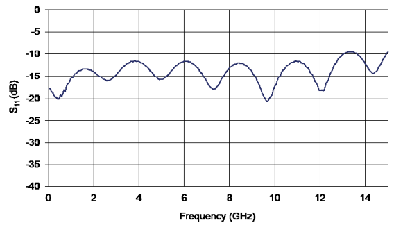
NIR-MX800-LN-20 Typical S_{11} Curve
