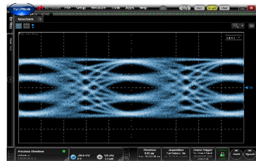
28 Gbauds PAM-4 eye diagram
