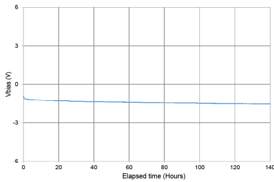
Modulator stability with time @25 °C and 80 mW
