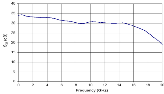
MXAN1300-LN-20 Typical S_{21} Curve
