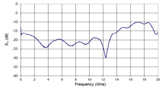
MXAN1300-LN-20 Typical S_{11} Curve
