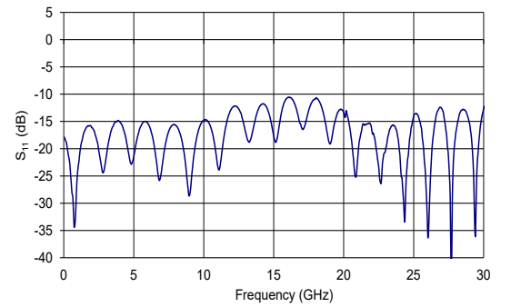
MX1300-LN-20 Typical S_{11} Curve
