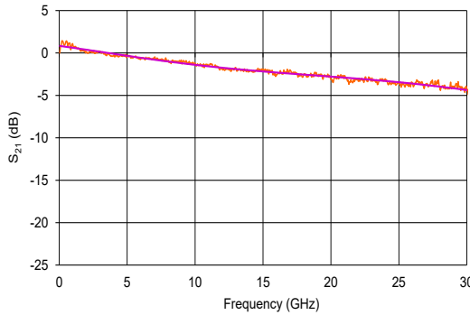
MX1300-LN-20 Typical S_{21} Curve
