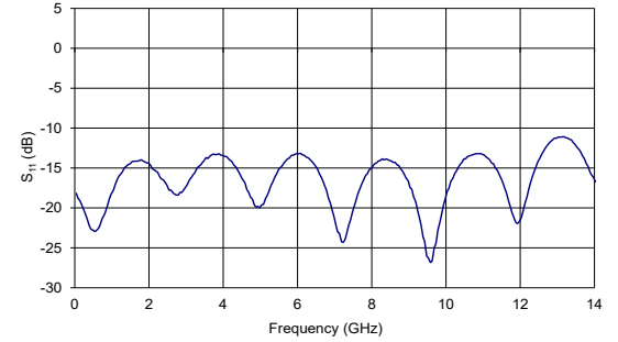
MX1300-LN-10 Typical S_{11} Curve
