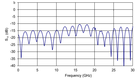
MX1300-LN-40 Typical S_{11} Curve
