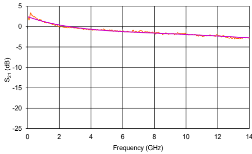
MX1300-LN-10 Typical S_{21} Curve
