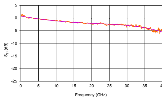
MX1300-LN-40 Typical S_{21} Curve
