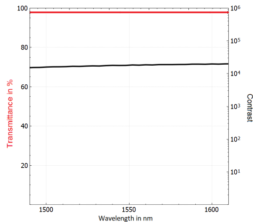
Typical contrast (black) and transmittance with AR-coating C1550 (red)
