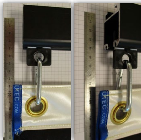
Rail profile
