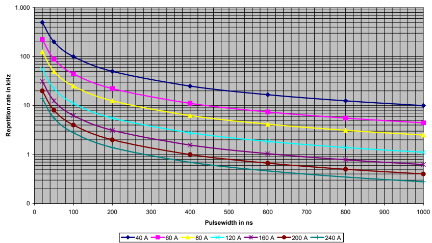
LDP-V 240-100 V3: Max. Reprate vs. Pulsewidths (internal HV, without cooling)
