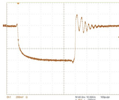
Figure: Current monitor output, scale: -80 A/Div
