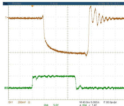
Typical trigger delay of LDP-V 240-100
