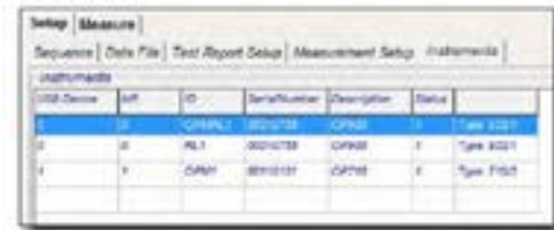
Figure 4: Instruments tab in setup
