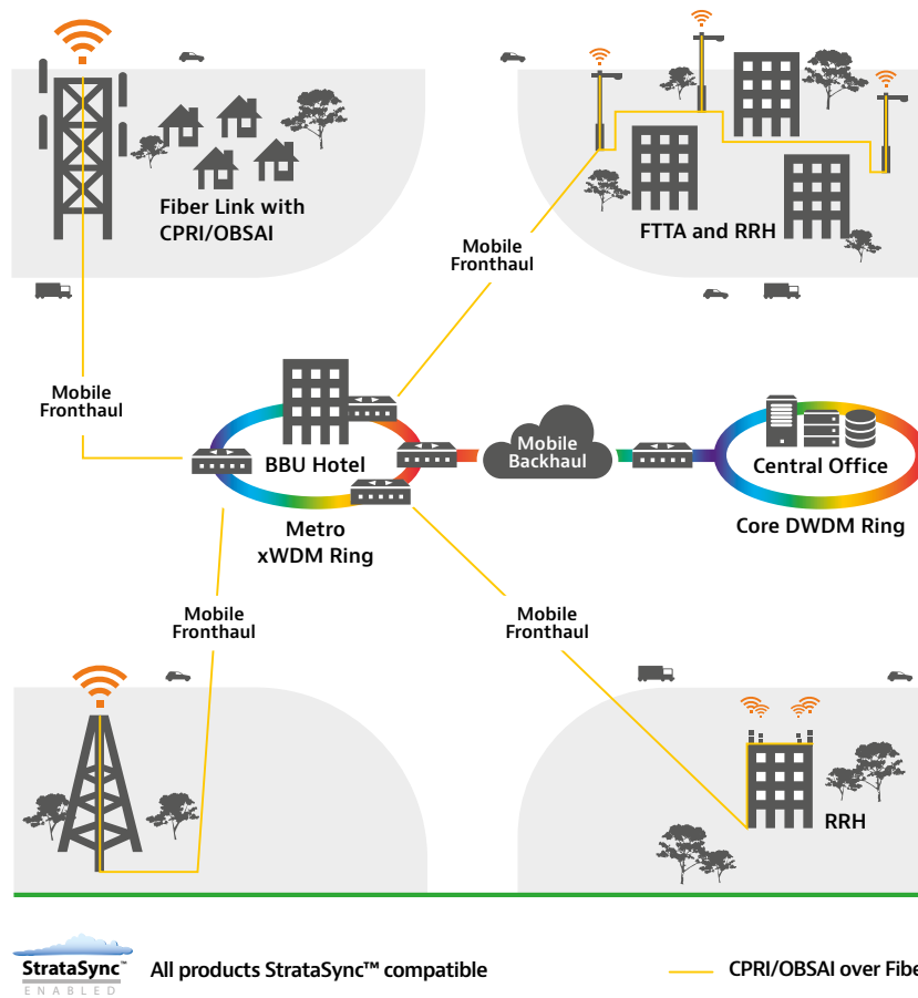
Figure 3: Centralized Radio Access Network (C-RAN)
