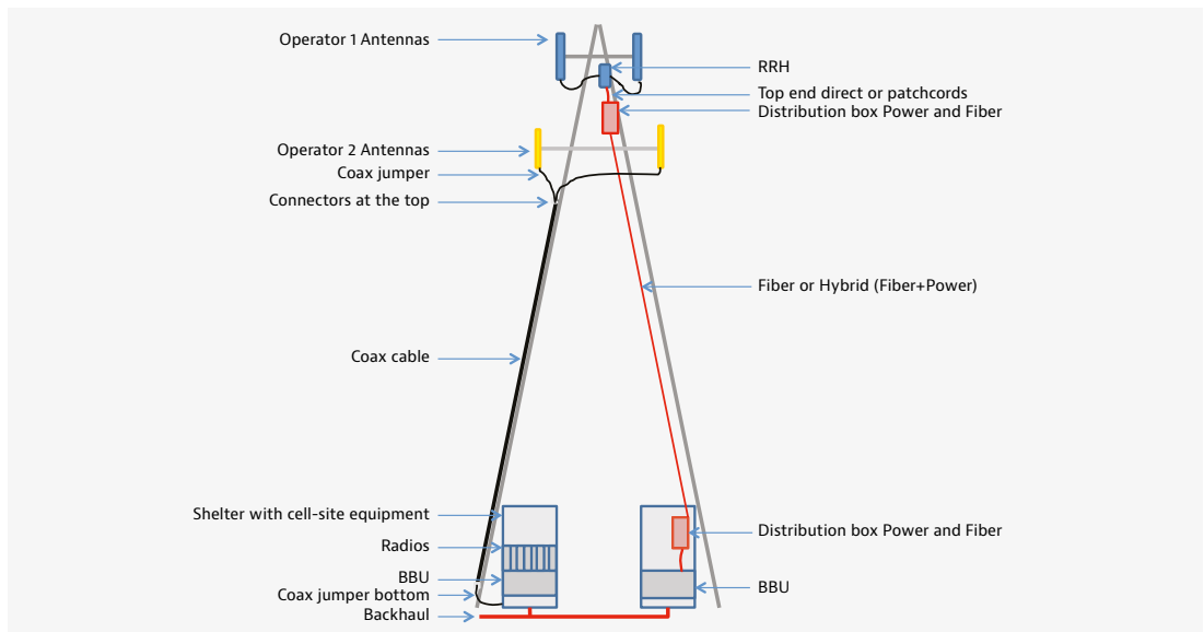
Figure 1: Common cell site structure and components
