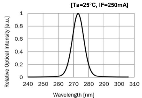
FIG 4. Typical Spectrum
