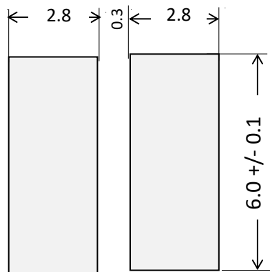
Recommended Solder Pattern on PCB
