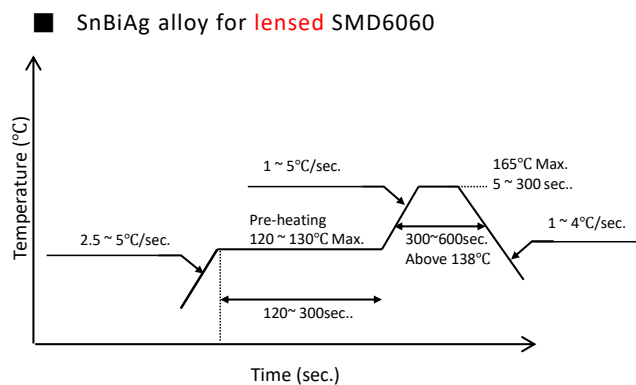
FIG 8. Solder reflow temperature profile
