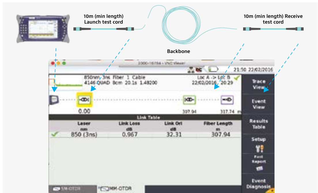
Figure 15. OTDR traces today present in a schematic view. By tapping on one of the events you can see reflectance of that particular event.
