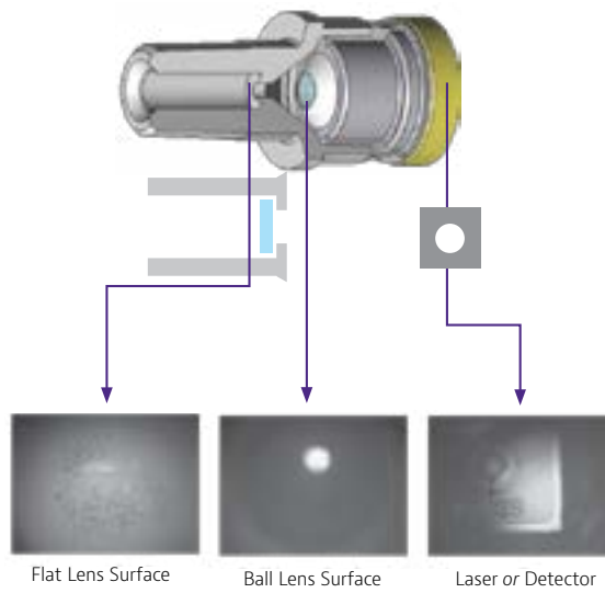
Figure 11 – Example views of Elements within PC Lens Type Transceivers
