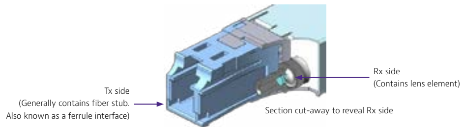
Figure 3. SFP Transceiver Cut-away View
