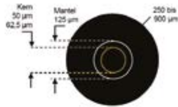
Multimode Fiber Dimensions
