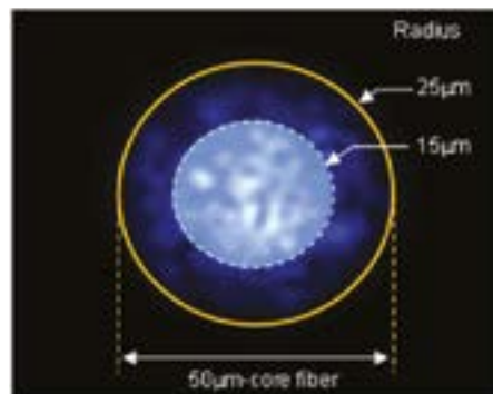
Illustration of EF value at 15 \mu\text{m} radius of a 50 \mu\text{m} -core fiber
