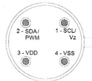
Figure 4. Package Top View
