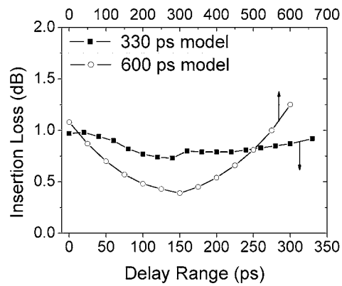
Figure 1. Insertion loss vs. optical delay.
