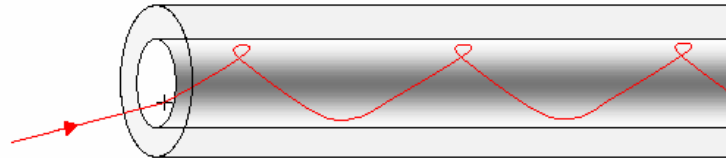
Figure 2: Skew ray in a graded-index fibre.
