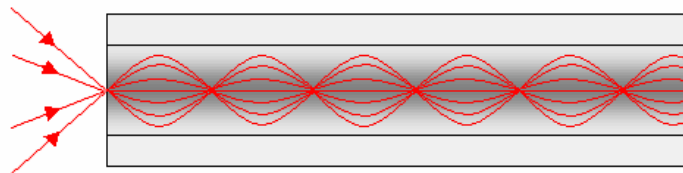
Figure 1: Meridional rays in a graded-index fibre.
