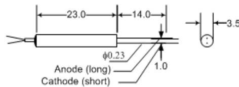
Directional package
