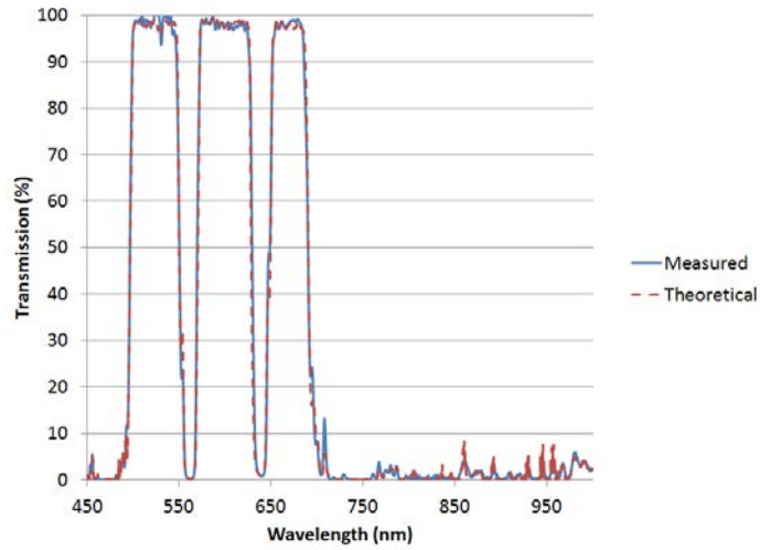
Figure 3. Triple bandpass polychroic on a 1.0 mm thick fused silica substrate with measured flatness of < 0.25 Waves / inch RMS @ 632.8 nm.
