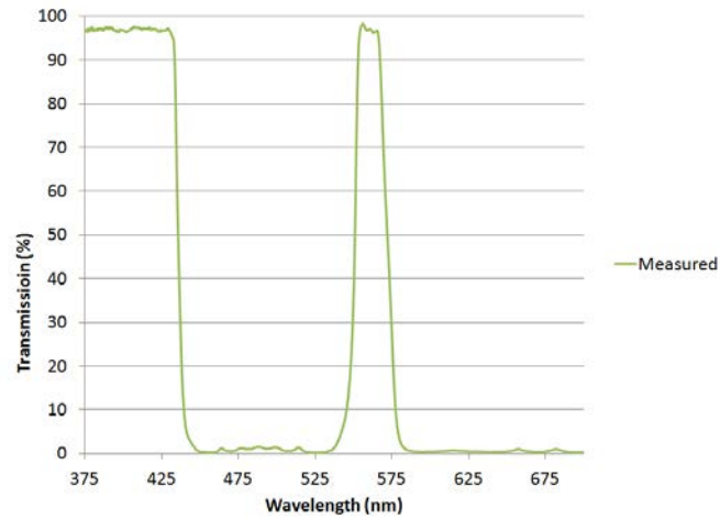
Figure 4. Dual notch polychroic on a 0.5 mm thick fused silica substrate with measured flatness of < 0.25 Waves / inch RMS @ 632.8 nm.
