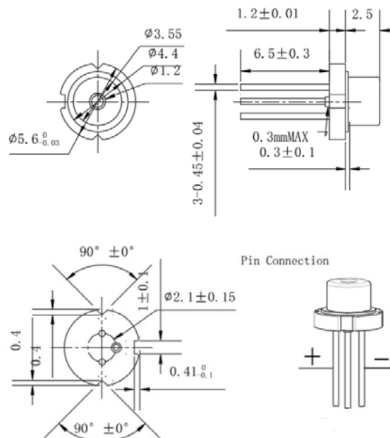
VD-0808I-300M-5H-2A0 with Substrate 5= NiFe and Package H= TO56 (unit: mm)
