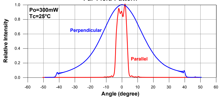
Far-Field Pattern
