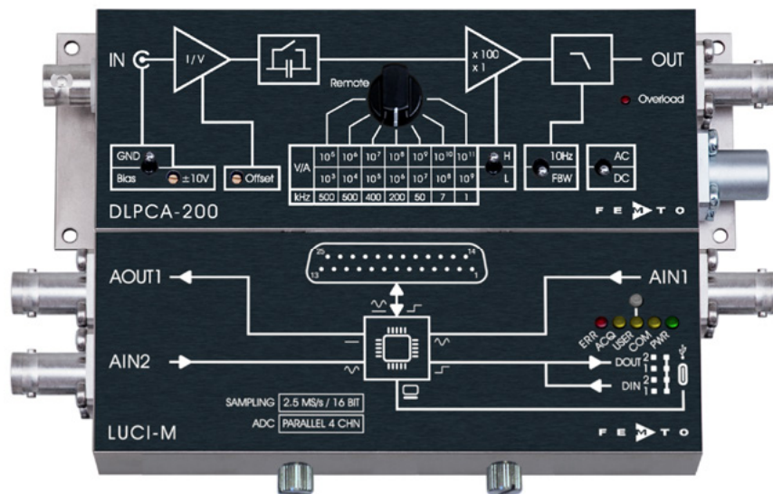
Application example: LUCI-M connected to DPCA-200
