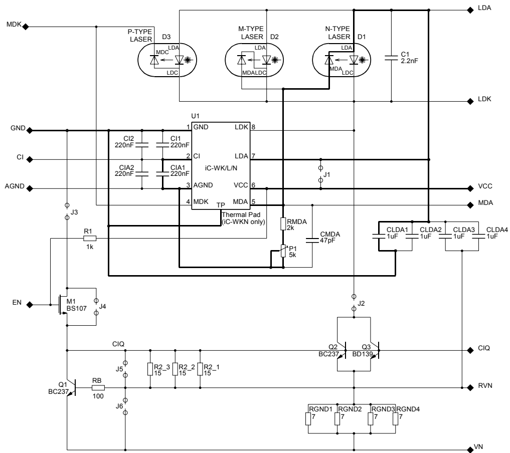
Figure 2: Schematic diagram of WK4D board (default configuration highlighted).
