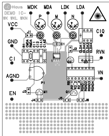
Figure 1: Component side of WK4D board
