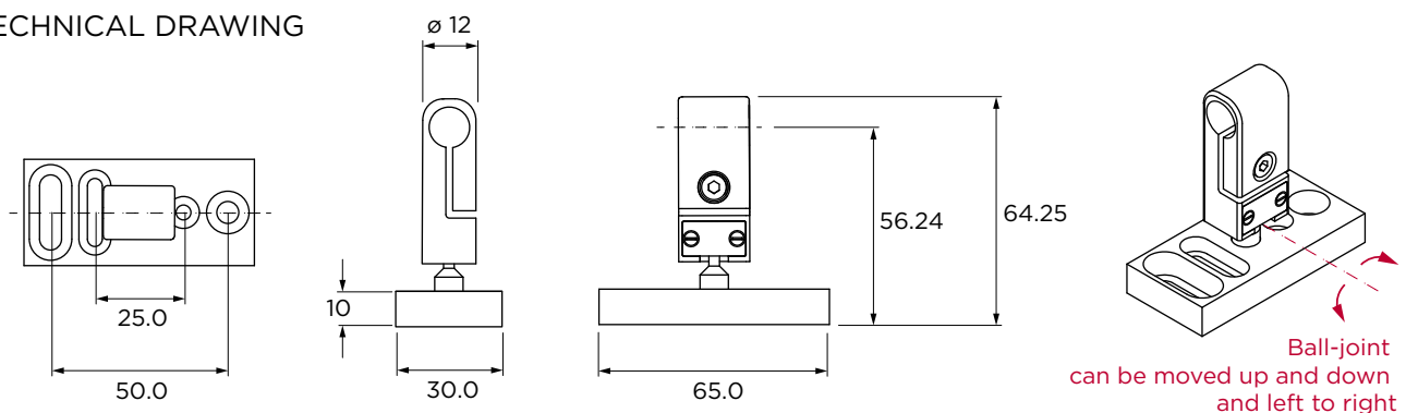
FP-MG-11.5 Mount
