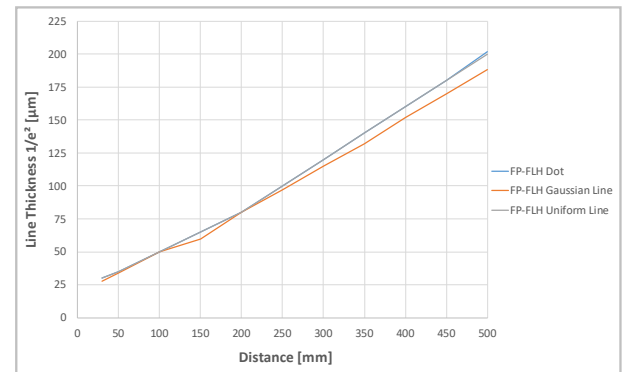
Fig. 8: Line thickness nearfield ( P = 0 \dots 30 mW)
