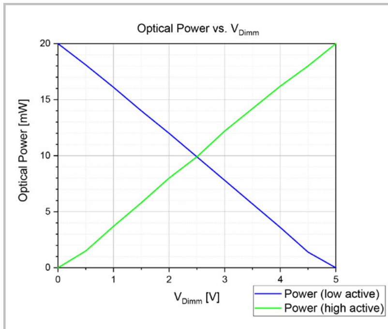
Fig. 6: Typical graph of an active high/active low logic for option D/DI (dimmmable)
