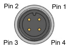
Fig.5: M12 connector, laser side
