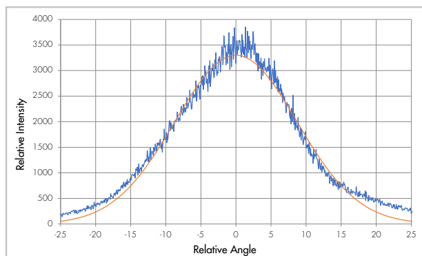
Figure 9: Relative Divergence Fast Axis
