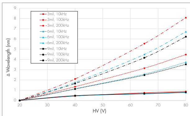
Figure 5: \Delta Wavelength vs HV, T_{case} = 21\text{ °C}
