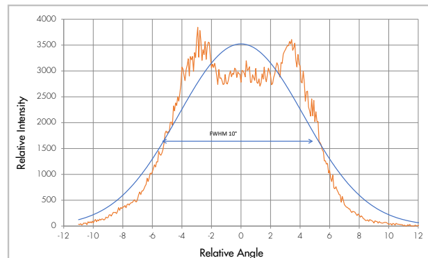
Figure 10: Relative Divergence Slow Axis
