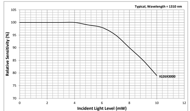
Fig. 9: Linearity
