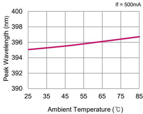
■ Ambient Temperature vs. Peak Wavelength
