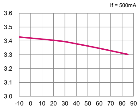
■ Ambient Temperature vs. Forward Voltage
