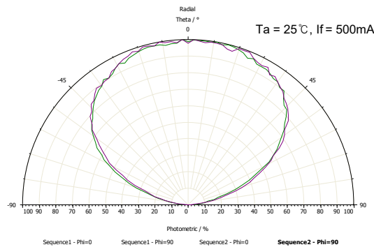
■ Radiation Characteristics
