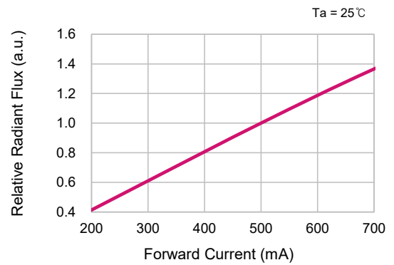
■ Forward Current vs. Relative Radiant Flux
