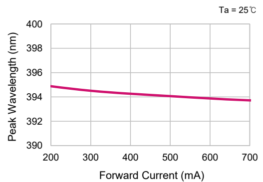
■ Forward Current vs. Peak Wavelength
