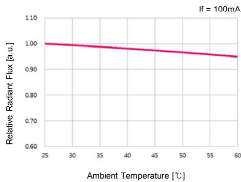
▪ Ambient Temperature vs. Relative Radiant Flux
