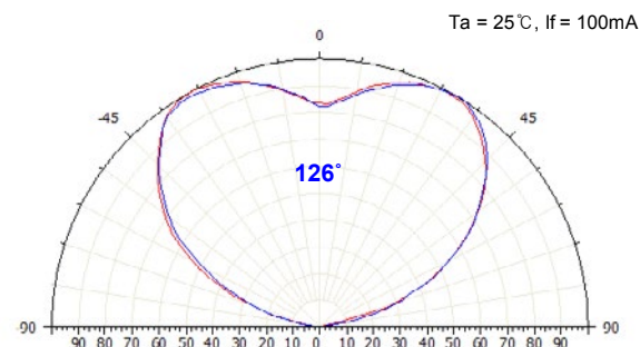
▪ Radiation Characteristics
