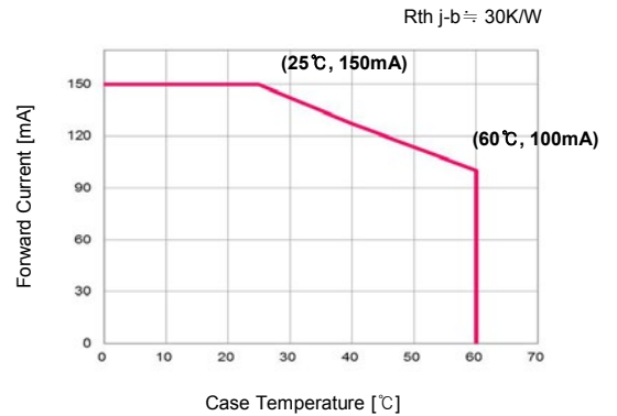
▪ Derating Curve
