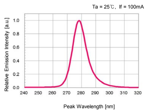
▪ Spectrum
