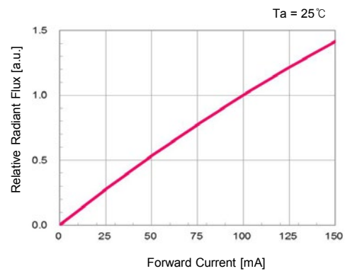
▪ Forward Current vs. Relative Radiant Flux
