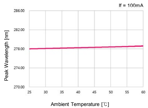
▪ Ambient Temperature vs. Peak Wavelength
