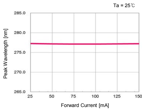
▪ Forward Current vs. Peak Wavelength
