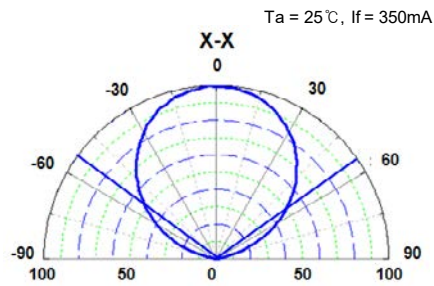
▪ Radiation Characteristics (Angle of Beam Spread, Directivity)
