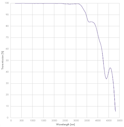
Interne Transmission Corning 7979 (Dicke: 3 mm)
